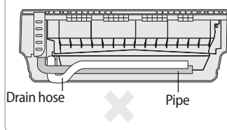
2) Incorrect connection
